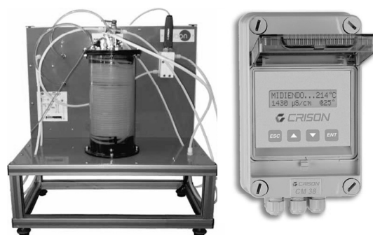
Fig. 2 PFR and Conductivity meter
