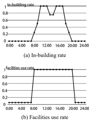
Fig. 6 Work mode in workdays of office buildings
