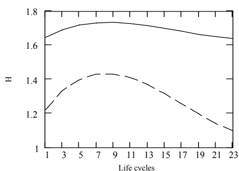
Fig. 6 Dynamics (trends) entropy function H .
