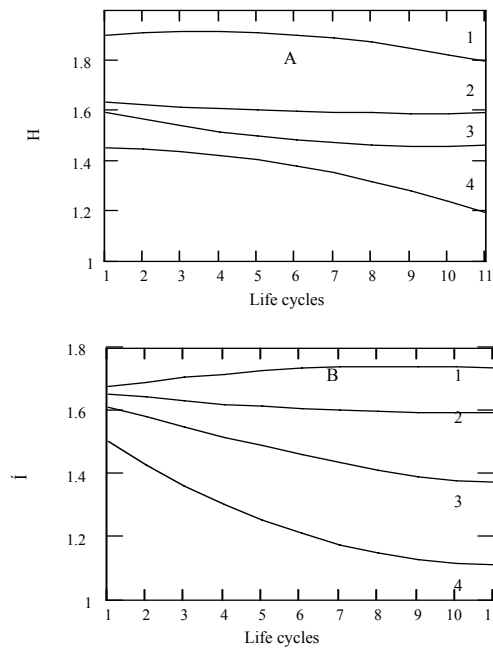
Fig. 5 Dynamics of entropy function for chemical elements composition of the plant tissues. A – tomato cultivated on granite crush stone, B – tomato cultivated on zeolite. 1 - roots, 2 – leaves, 3 – stems, 4 – fruits
