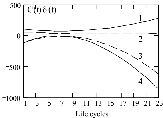
Fig. 4 Dynamics of the information streams C(t) . 1, 2 – roots ( X ) \rightarrow reproductive bodies ( Y ). 3, 4 – roots ( X ) \leftarrow stems ( Y ). ——— spring wheat, - - - - - tomato
