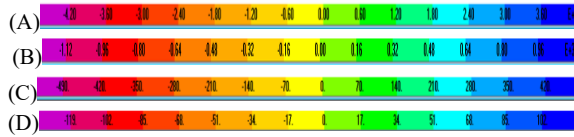
Fig. 19 Internal force diagram of \circ, A axis wall in +X direction wind load case
