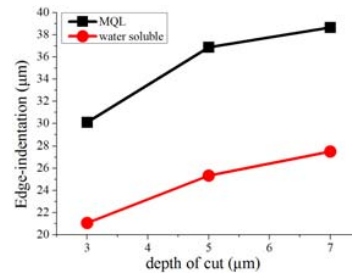
(a) V=565 m/min
