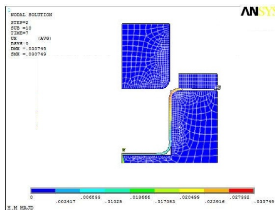
Fig.2 FEM simulation
