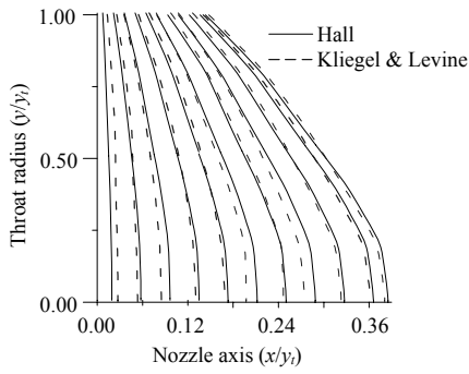
Fig. 3 Nozzle 1 throat region isobars
