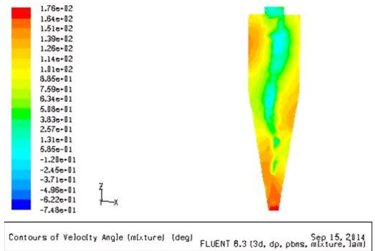
Fig. 10 Velocity direction within the hydrocyclone
