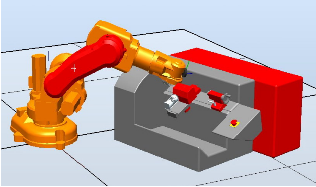
Fig. 1 Computer model of the workcell with ABB 140 robot
