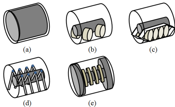
Fig. 1 Classification of in-pipe robots : (a) PIG type, (b) Wheel type, (c) Track type, (d) Walking type, (e) Inchworm type
