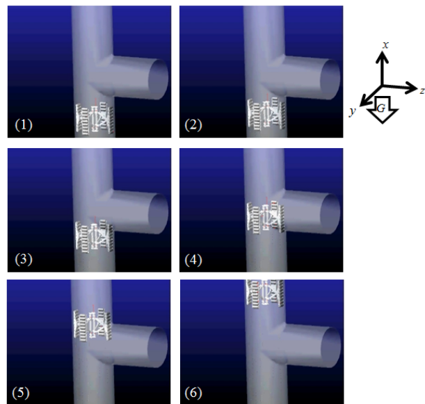
Fig. 7 Simulation results with x-axis gravity
