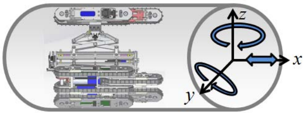
Fig. 3 Translation and rotation required for in-pipe robot inside pipelines to move freely
