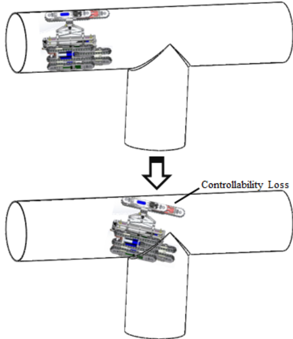
Fig. 4 Instant moment of an in-pipe robot crossing branched section
