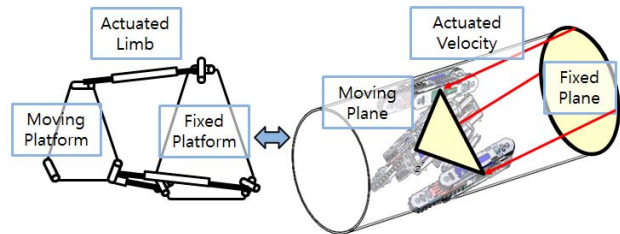
Fig. 2 Analogousness between parallel manipulator and three legged in-pipe robot
