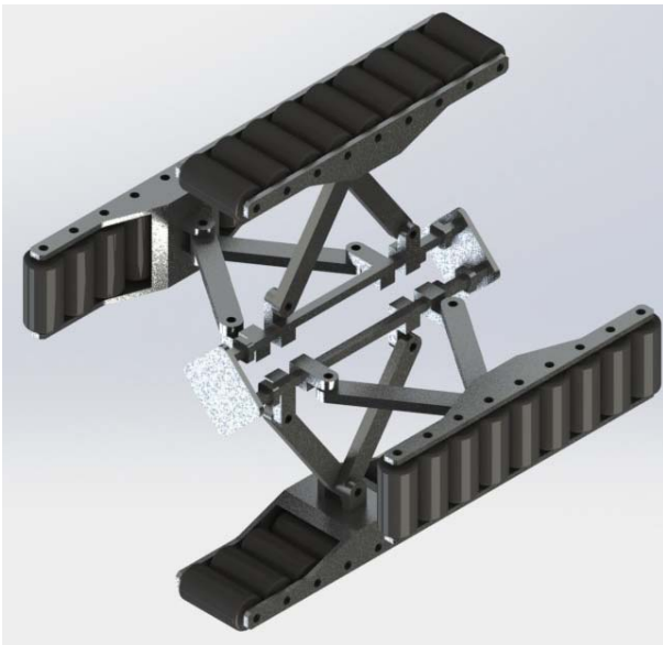
Fig. 6 Simplified model of newly proposed design
