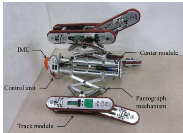
Fig. 5 Configuration of PAROYS
