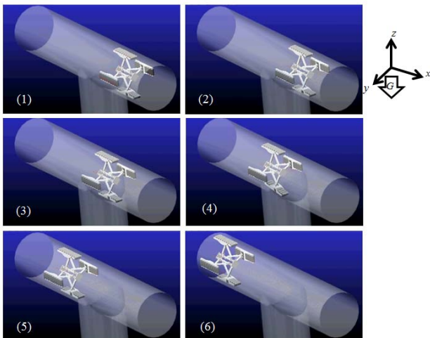
Fig. 8 Simulation results with z-axis gravity
