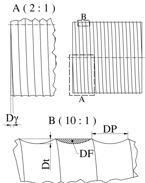
Fig. 1 The parameters of twist measurement
