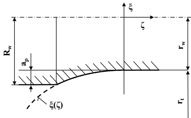
Fig. 3 Illustration of the cut surface equation
