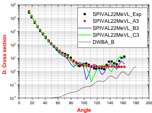
Fig. 4 Comparison between the experimental and the calculated angular distribution within the energy frame work of DWBA and SPIVAL at 22 MeV
