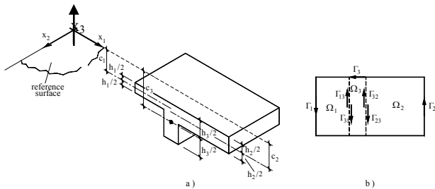
Fig. 1 (a) General zoned plate domain; (b) reference surface view
