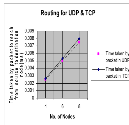
Fig. 4 Time Taken by a packet from source to destination node for UDP &amp; TCP Protocols w.r.t. no. of nodes
