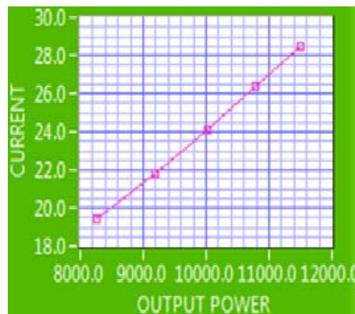
Fig. 7 Current vs output Power
