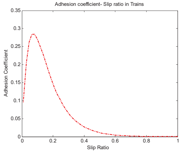
Fig. 2 Relation between adhesion coefficient and slip ratio
