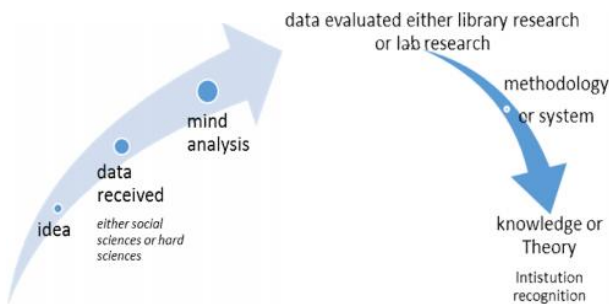
Fig. 3 Data process
