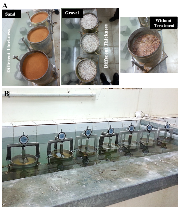
Fig. 6 Seven undisturbed shale molds (6 treatments and 1 without) with different type and thickness of replacement CCS used for treatment (A); seven molds submerged in a water tank and fixed a dial gage (0.01mm) for measurement of swelling (B); Al Qadsiyah district, Tabuk, KSA
