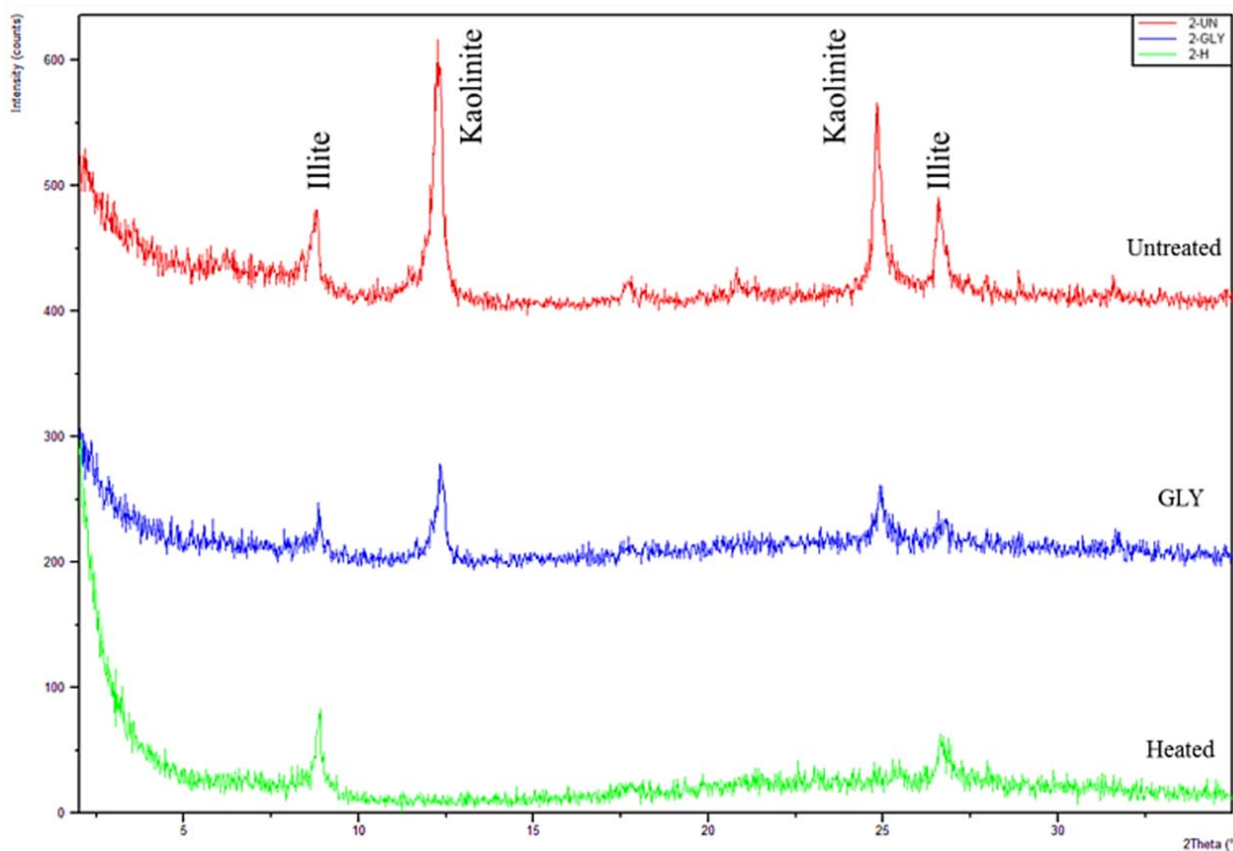
Fig. 4 Completed signal quantification with labeled peaks of expansive Tabuk shale, Al Qadsiyah district, Tabuk, KSA
