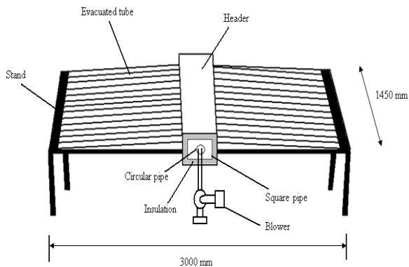
Fig.1 Schematic of solar air heating based on evacuated tube solar collector
