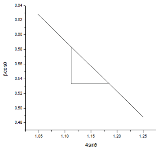
Fig. 2 Williamson-Hall plot
