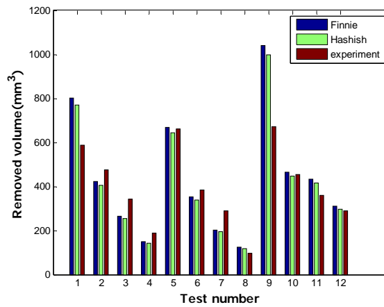
Fig. 4 Material removed predicted by Finnie and Hashish models
