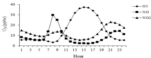
Fig. 1 Diurnal variation of O 3 , NO and NO 2 recorded at Putrajaya (S1), Petaling Jaya (S2) and Nilai (S3) stations
