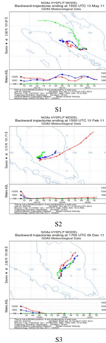
Fig. 4 Backward trajectory of wind direction for the Putrajaya (S1), Petaling Jaya (S2) and Nilai (S3) monitoring stations for the highest O 3 episode in 2011
