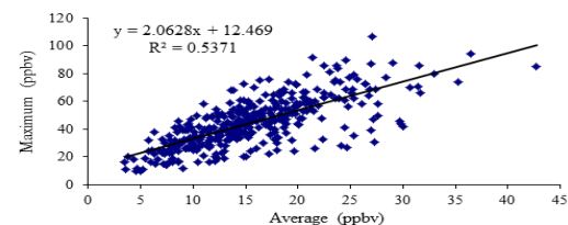
Fig. 2 Average and daily maximum variations of ozone concentration at Putrajaya (S1), Petaling Jaya (S2) and Nilai (S3) stations
