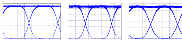
(a) Q = 40 dB (b) Q = 38 dB (c) Q = 36.6 dB
