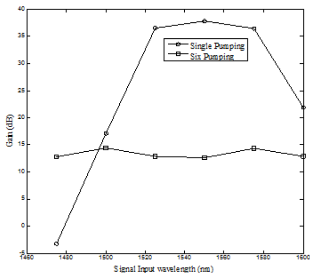
Fig. 4 Variation of Raman gain for eight spans of Raman fiber length of 10 km
