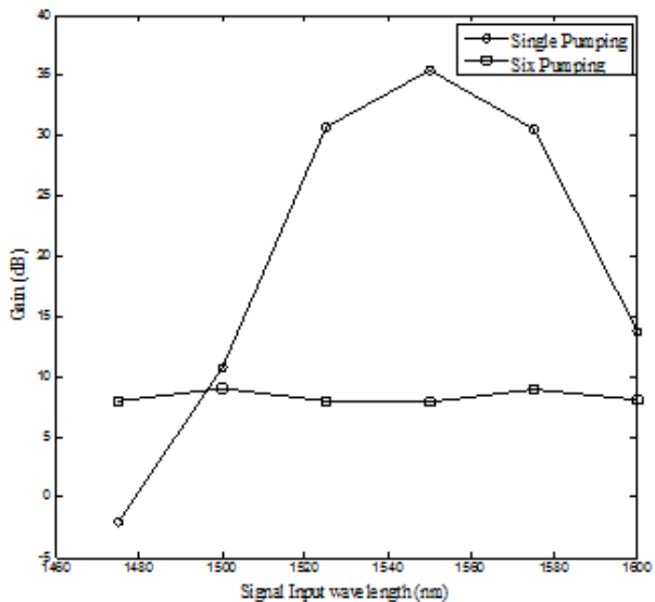
Fig. 3 Variation of Raman gain for five spans of Raman fiber length of 10 km
