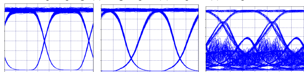
(a) Q = 34.6 dB (b) Q = 38.4 dB (c) Q = 6 dB
