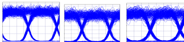
(a) Q = 23 dB (b) Q = 21 dB (c) Q = 19.8 dB
