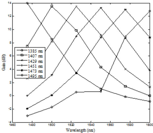
Fig. 1 Gain contribution from individual pump wavelengths
