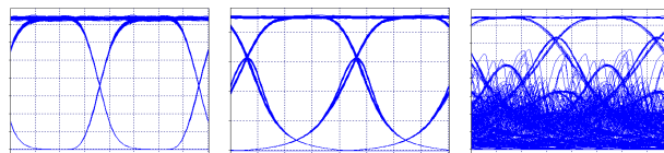
(a) Q = 40 dB (b) Q = 15.2 dB (c) Q = 6 dB
