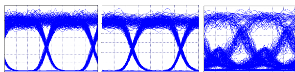
(a) Q = 23.8 dB (b) Q = 23.85 dB (c) Q = 6 dB
