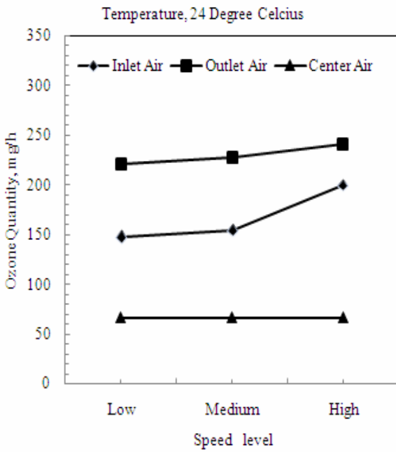
Fig. 4 Ozone Quantity vs Plasma Generator Position and Speed Level (24 Degree)
