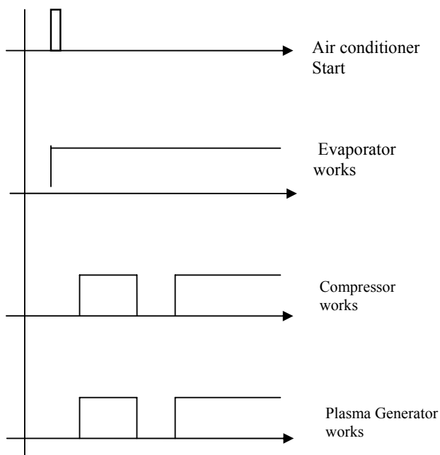
Fig. 2 Arc Timing Diagram
