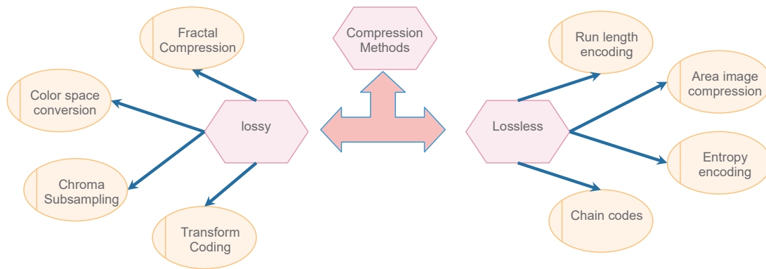
Fig. 1 Compression Methods
