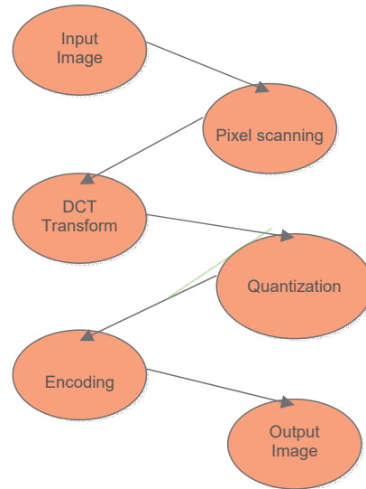
Fig. 2 JPEG Compression
