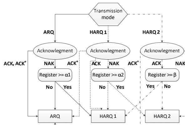
Fig. 2 Logic of transmitter in our proposal
