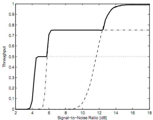
Fig. 5 Dependence of relative throughput on SNR
