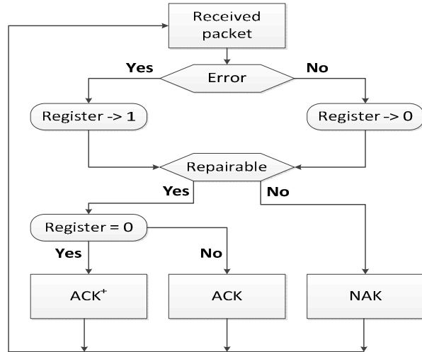
Fig. 1 Logic of receiver in our proposal
