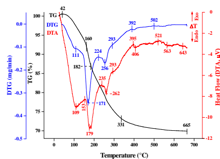
Fig. 4 Thermal analysis of \text{Cu-Mn}/\gamma\text{-Al}_2\text{O}_3 (1:5). Active component content 21.0%
