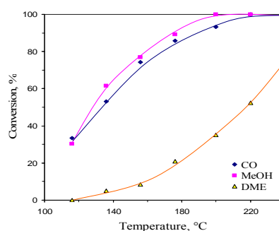
Fig. 12 Temperature dependence of CO, \text{CH}_3\text{OH} and DME conversion over Cu-Mn/ \gamma - \text{Al}_2\text{O}_3 catalyst with Cu/Mn molar ratio 2:1
