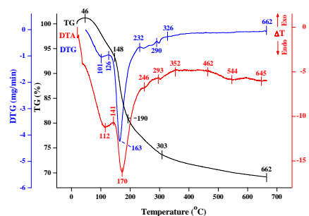
Fig. 5 Thermal analysis of \text{Cu-Mn}/\gamma\text{-Al}_2\text{O}_3 (2:1). Active component content 21.0%
