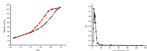
Fig. 7 Adsorption-desorption isotherm and pore size distribution of Cu-Mn 1:5 (S BET =152 m 2 .g -1 )
