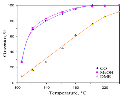
Fig. 13 Temperature dependence of CO, CH 3 OH and DME conversion over Cu-Mn/ \gamma -Al 2 O 3 catalyst with Cu/Mn molar ratio 1:5
