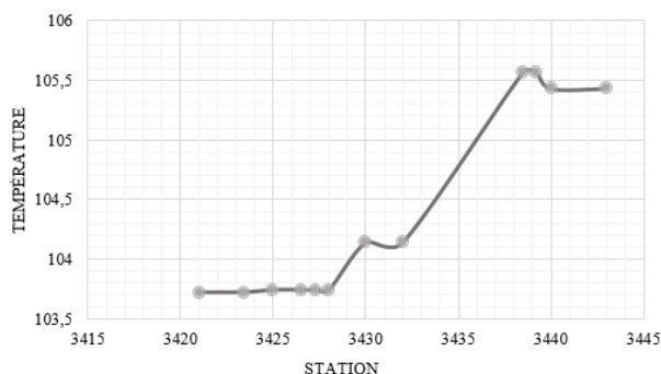
Fig. 5 Evolution of the temperature according to the different levels of the productive layer
