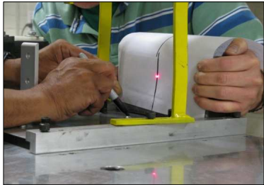
Fig. 1 Laser beam adjustment with collimator device
