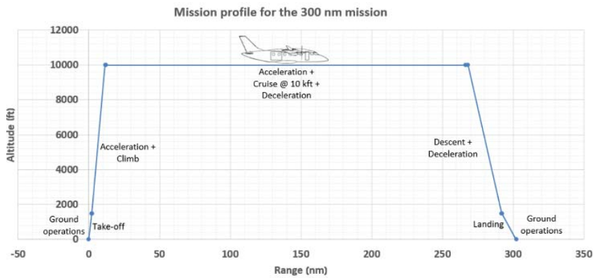
Fig. 5 Design mission
