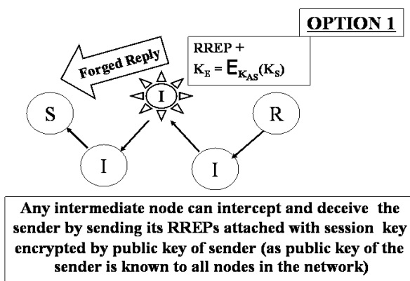
Fig. 4 Forged RREP from an intermediate node
