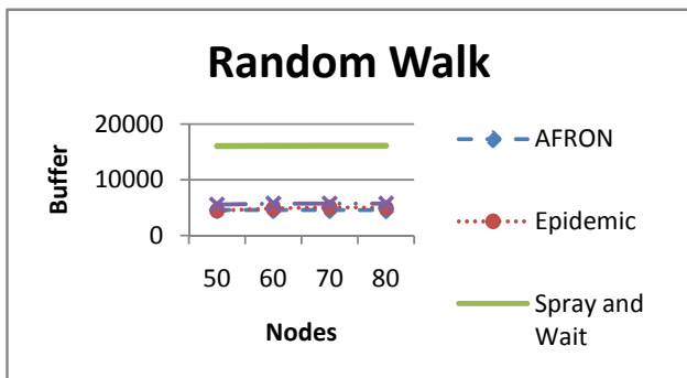
Fig. 8 Buffer Consumption for Random Walk Scenario
