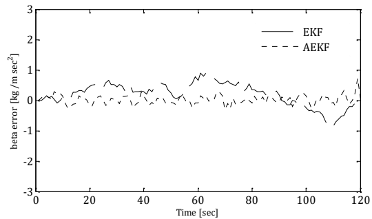
Fig. 10 Error of EKF (dashed line) and AEKF (dotted-line) for beta estimation
