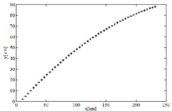
Fig. 3 Trajectory of BM
