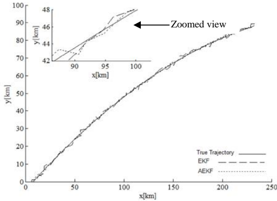
Fig. 7 Estimated Trajectory of BM
