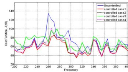
Fig. 8 Variation of the cost function with the location of the microphones
