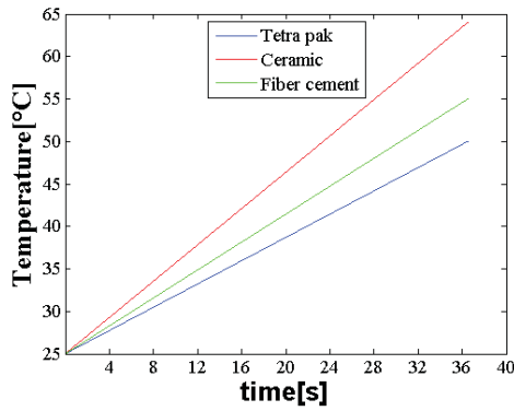
Fig. 2 Roof tiles temperature register
