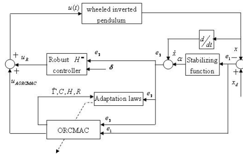
Fig. 2 Block diagram of RIBTC system
