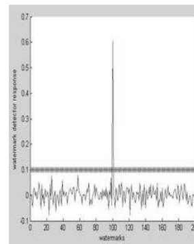
Fig. 32. Watermark detection response relating to the Video Object 3 (foreground) after format conversion from MPEG-4 to MPEG-2.
