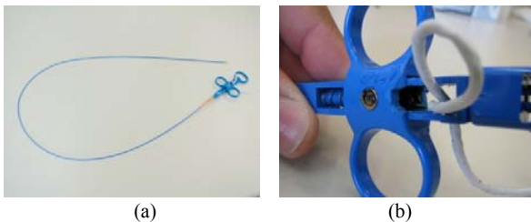
Fig. 3 (a) forceps; (b) detail of the electrical connection
