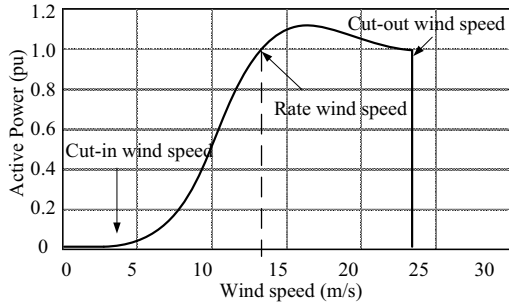
Fig. 2 The Power curve characteristic
