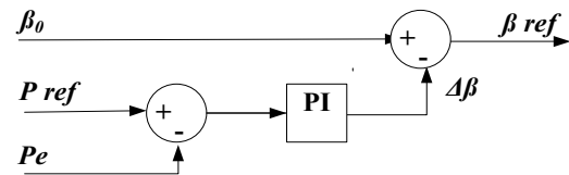
Fig. 8 The scheme of the pitch angle control system [16]
