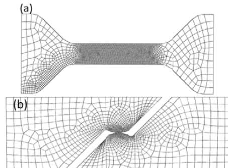
Fig. 8 Mesh of tensile and shear specimen
