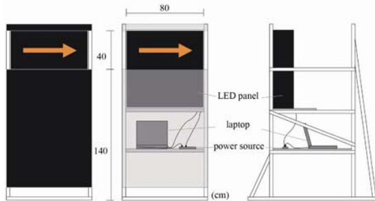
Fig. 3 Experimental equipment setup
