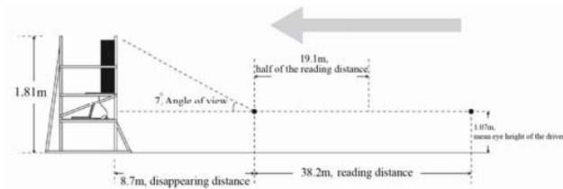
Fig. 2 Equipment setup range and visible distance
