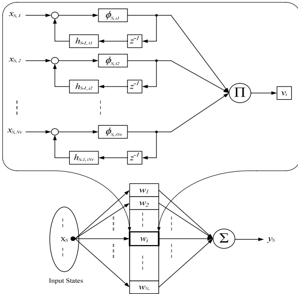
Fig. 1 RSCMAC structure
