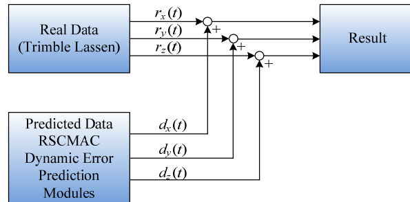
Fig. 8 GPS error improvement structure
