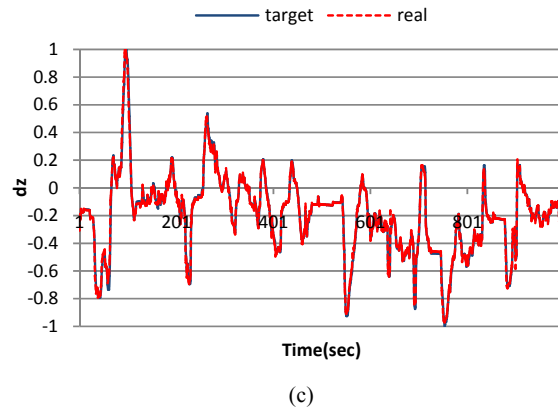
Fig. 7 RSCMAC dynamic prediction error test result
