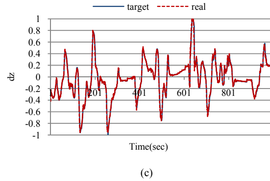
Fig. 5 RSCMAC dynamic error prediction training result
