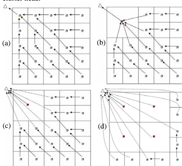
Fig. 7 The operation of cluster merging mechanism
