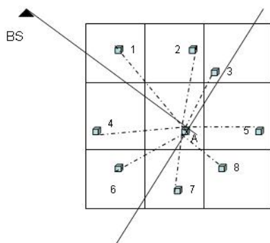
Fig. 5 Locating forwarding node in neighboring clusters
