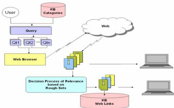
Fig. 6 Algorithm for the Classification model using the DPR-RS approach .
