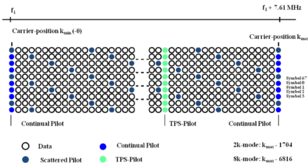
Fig. 5 Transmission Frame for the DVB-T signal [6]
