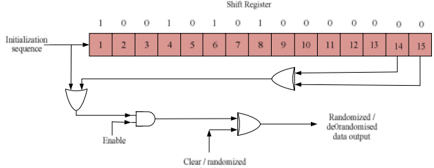
Fig. 3 Scrambler/Descrambler Schematic Diagram
