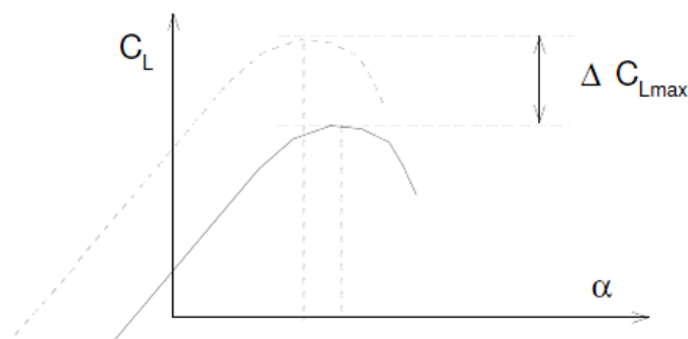
Fig. 2. Comparison between the lift curves for a wing with (dashed line) and without (continuous line) plain flaps.
