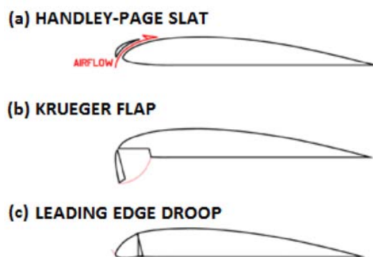
Fig. 8. A schematic representation of some leading edge devices.
