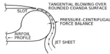
Fig. 9. A schematic representation of the CCW concept.
