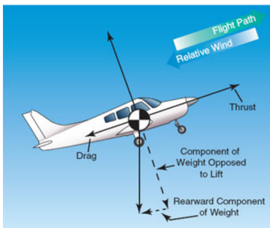
Fig. 1. Schematic representation of the aerodynamic forces acting on an aircraft during flight.
