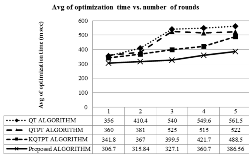
Fig. 11 Average of optimization time vs. number of rounds
