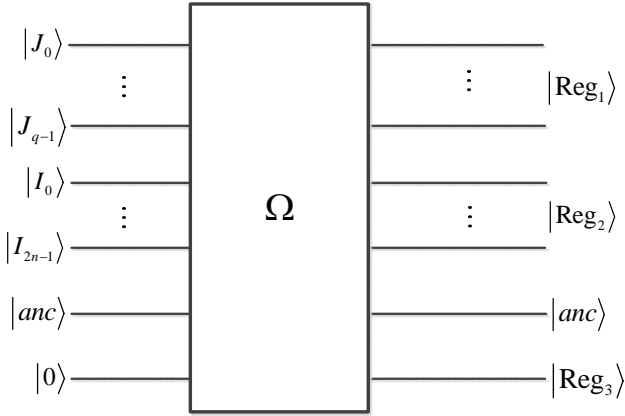
Fig. 3 The quantum accumulation \Omega
