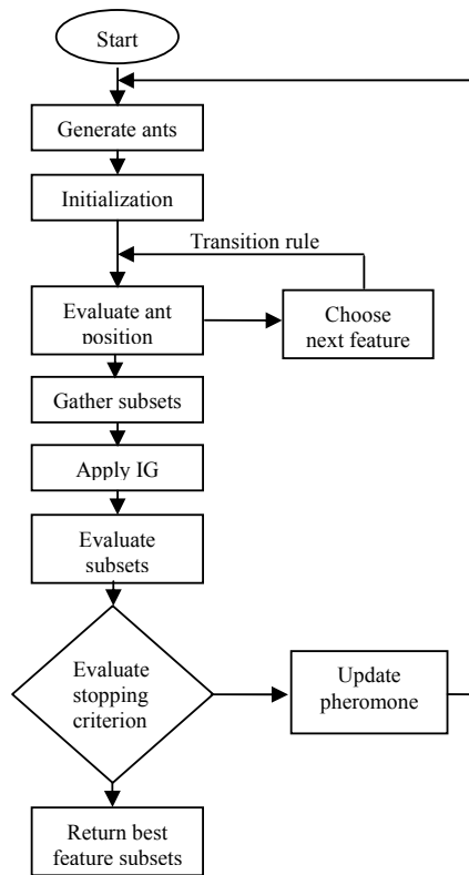
Fig. 3 Flow diagram of ACO-IG feature selection
