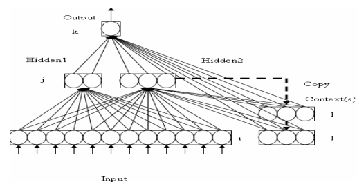
Fig. 1 The FFFB-MCANN Network
